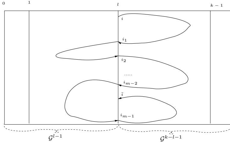
Fig. 2. Computing paths of weight (m_k^*)_{i^{(l)}, \overline{i^{(l)}}
