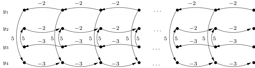
Fig. 3. Graph representation of \overline{R}^k , k = 1, 2, 3, \dots
